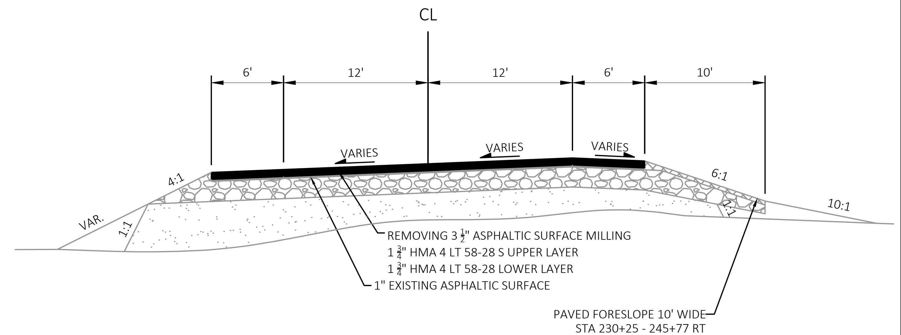
FINISHED TYPICAL SECTION
