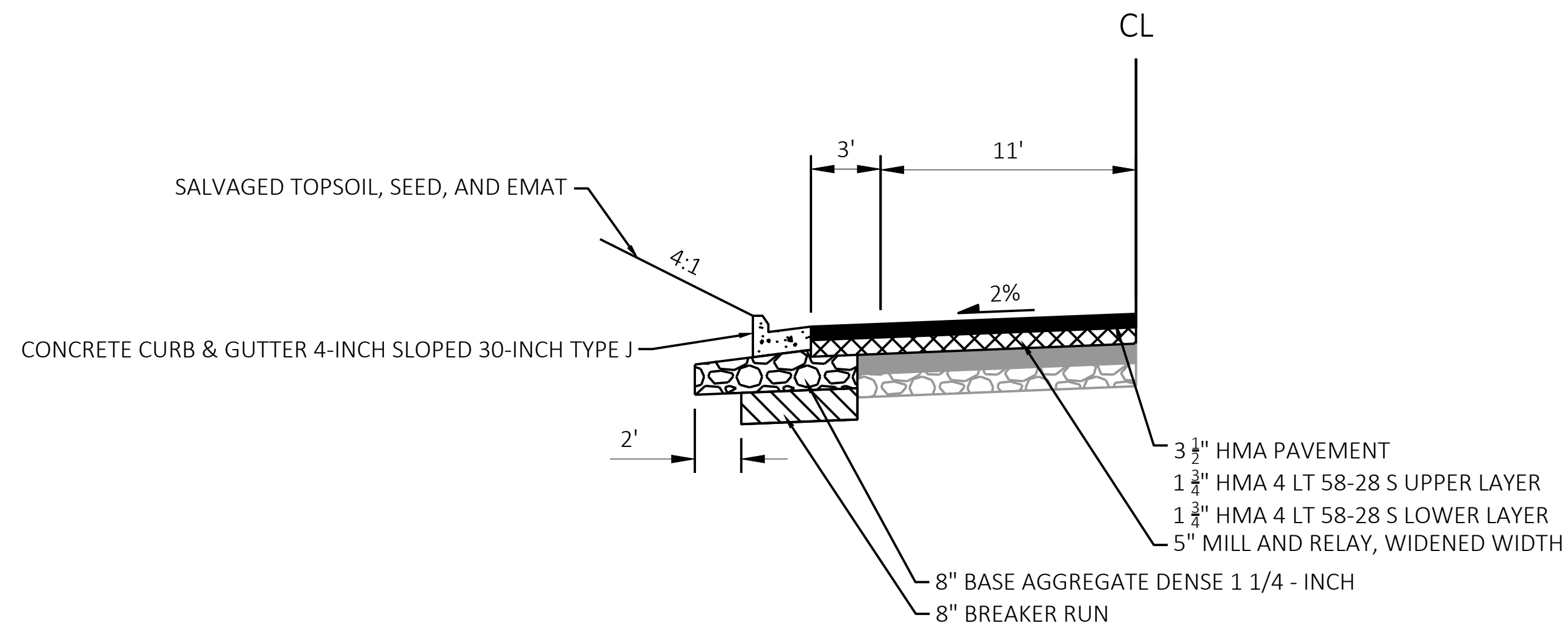
HALF FINISHED RURAL TYPICAL SECTION WITH CURB & GUTTER
