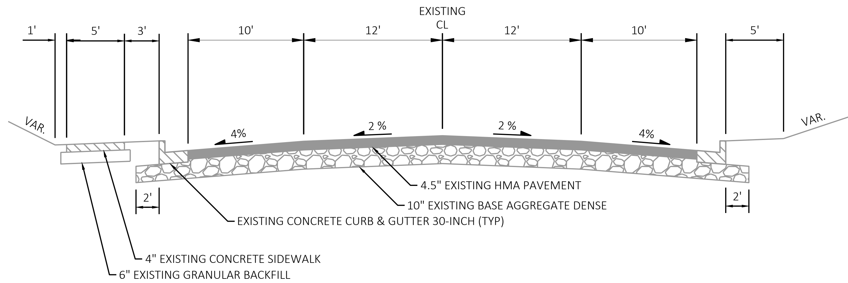
EXISTING URBAN TYPICAL SECTION
