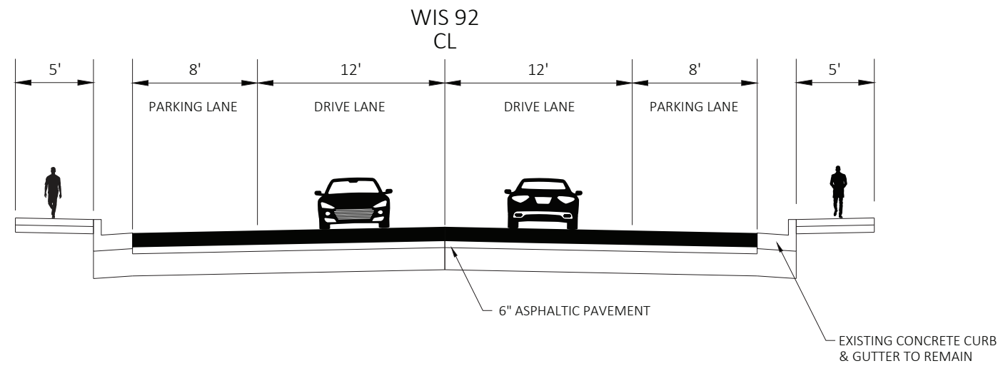
FINISHED TYPICAL SECTION ALASKA AVENUE TO EAST LINCOLN STREET
