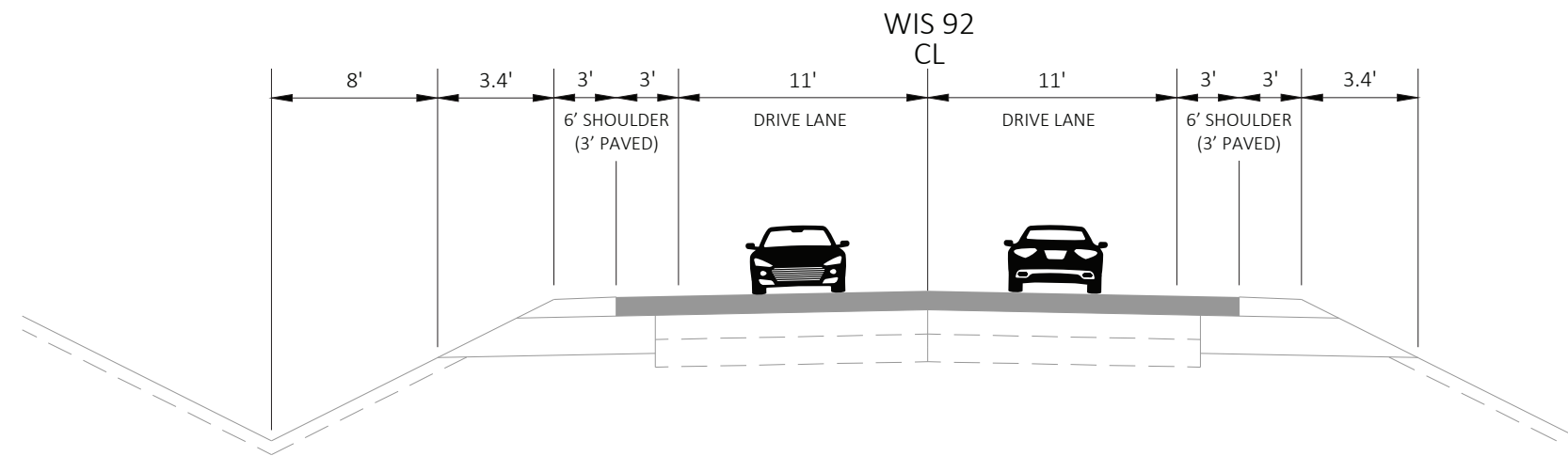
EXISTING TYPICAL SECTION EAST OF COUNTY JG TO STONEFIELD WAY
