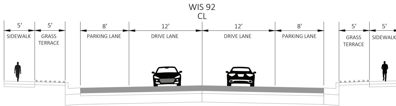
EXISTING TYPICAL SECTION EAST LINCOLN STREET TO EAST OF COUNTY JG
