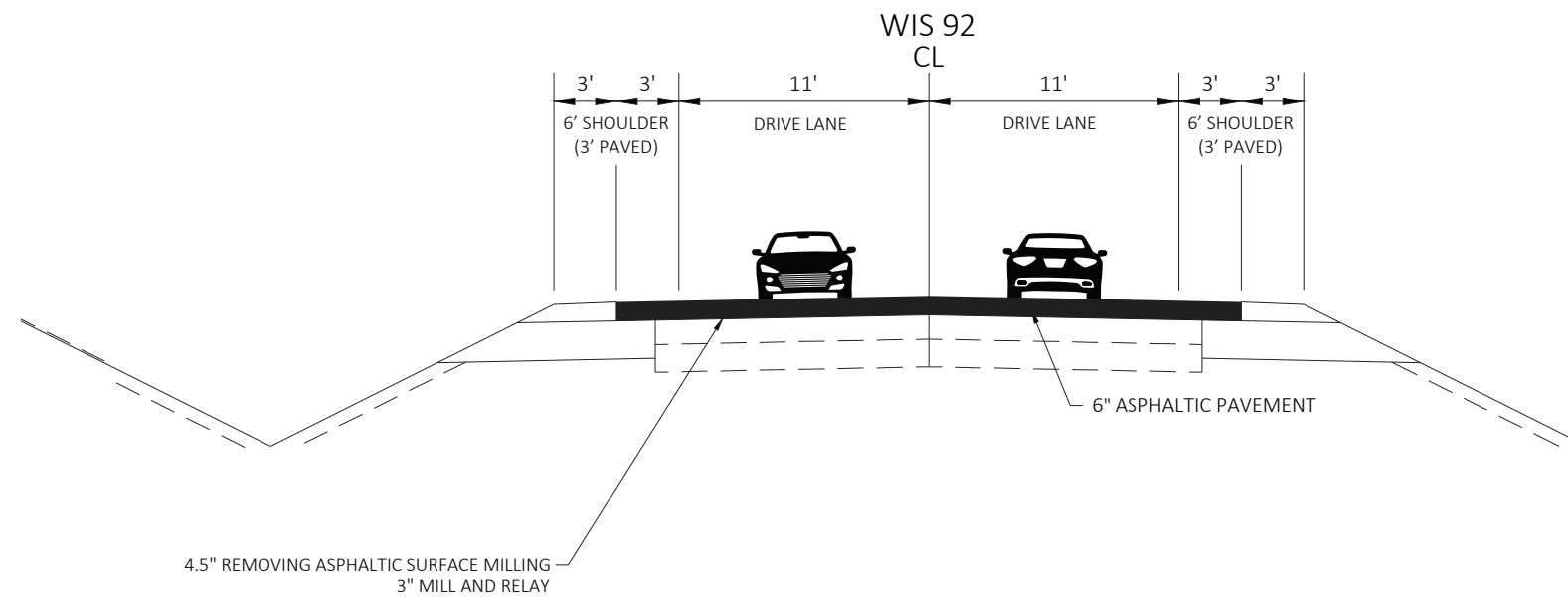
FINISHED TYPICAL SECTION EAST OF COUNTY JG TO STONEFIELD WAY
