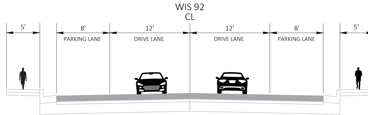
EXISTING TYPICAL SECTION ALASKA AVENUE TO EAST LINCOLN STREET
