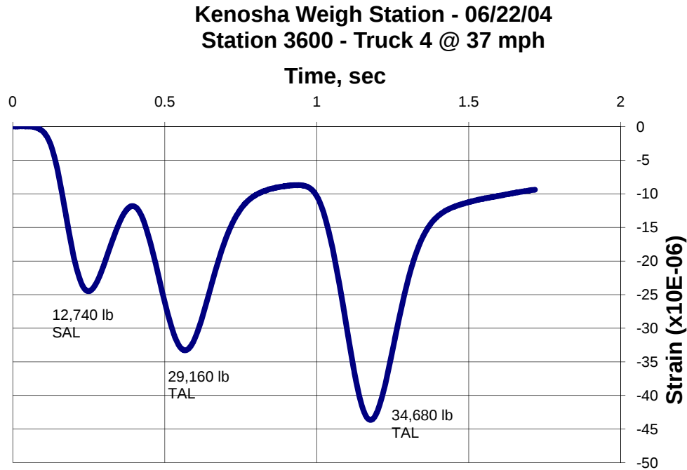
Figure 7: Strain Measurement from Truck 4 – June 2004
