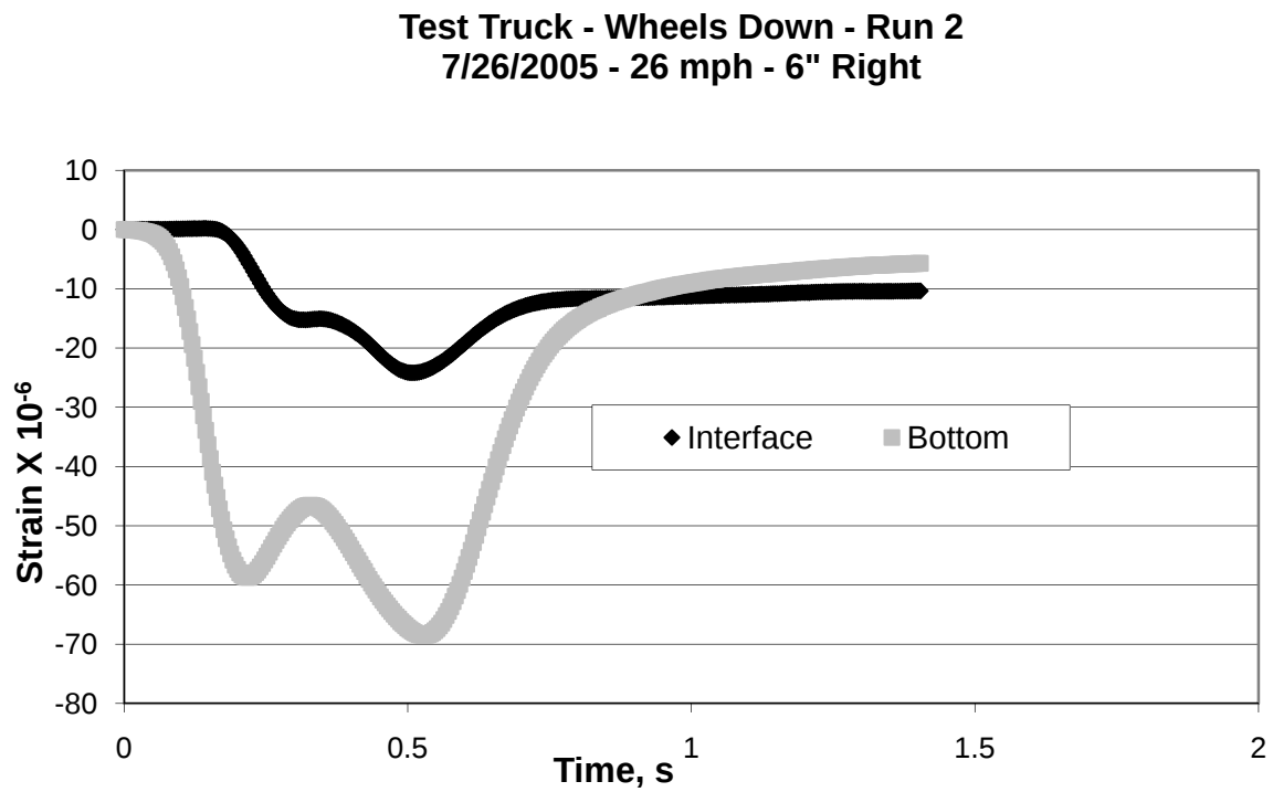
Figure 12: Strain Measurement from Truck Run 2 – July 2005
