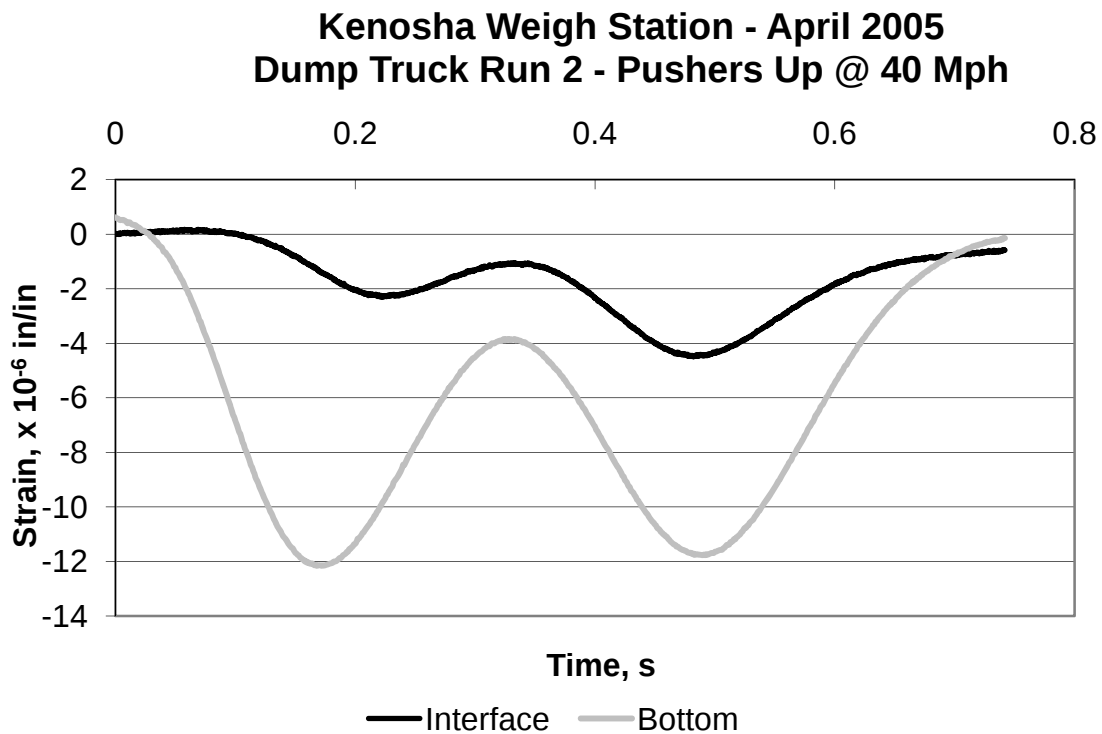
Figure 9: Strain Measurement from Truck Run 2 – April 2005
