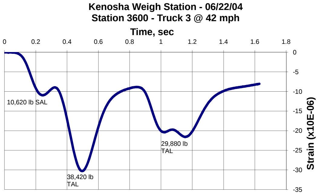
Figure 6: Strain Measurement from Truck 3 – June 2004
