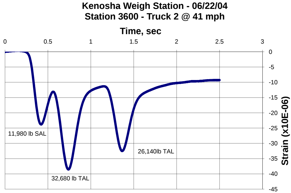
Figure 5: Strain Measurement from Truck 2 – June 2004
