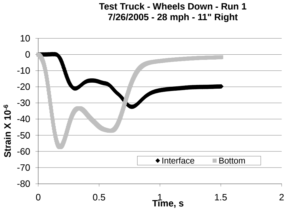
Figure 11: Strain Measurement from Truck Run 1 – July 2005
