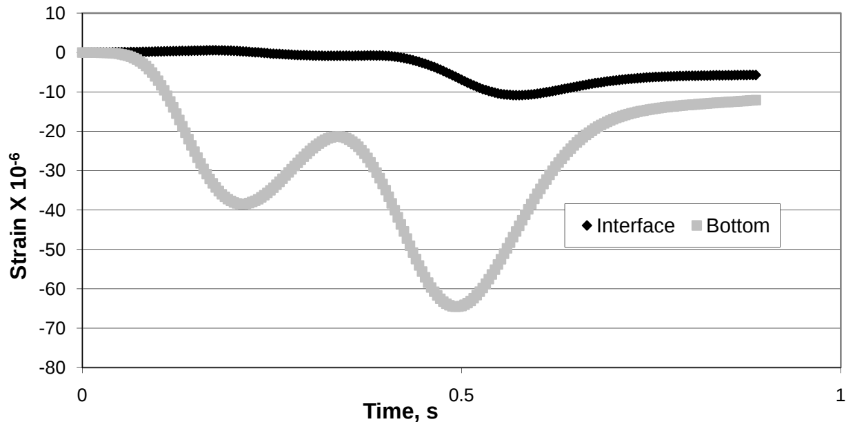
Figure 17: Strain Measurement from Truck Run 7 – July 2005
