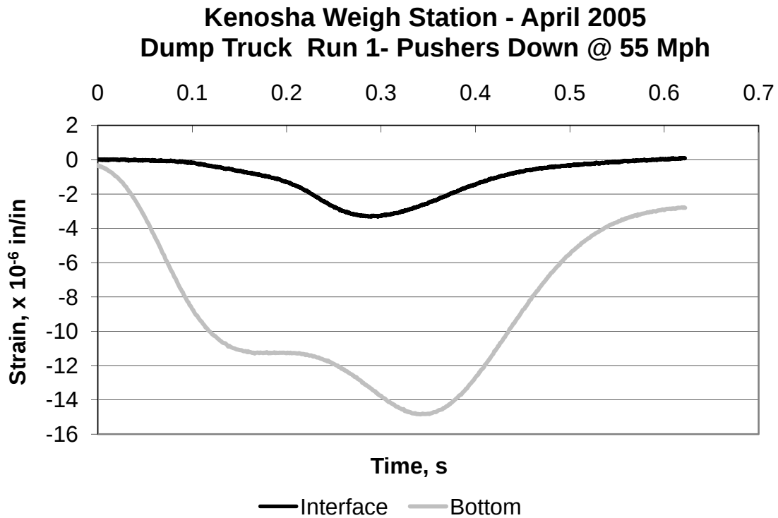
Figure 8: Strain Measurement from Truck Run 1 – April 2005
