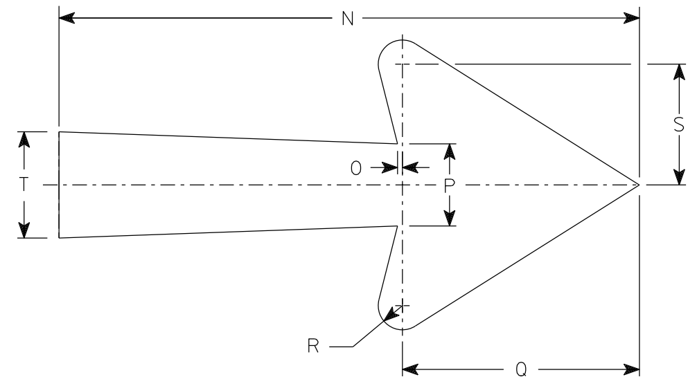
Arrow Detail
