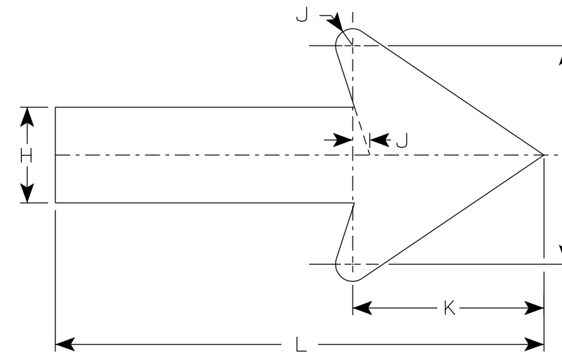
ARROW DETAIL
