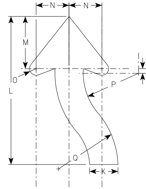
ARROW DETAIL
