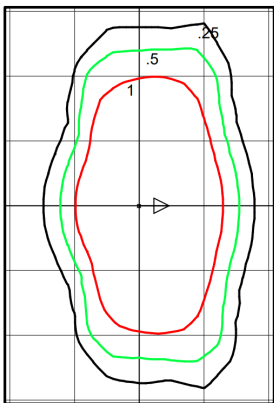
24L 4000K (TYPE II)
