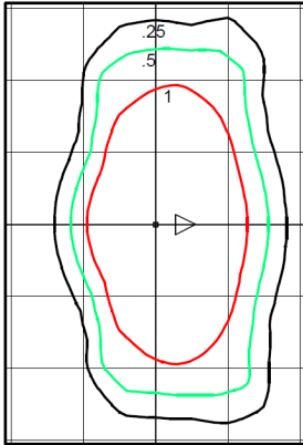
15L 4000K (TYPE II)
