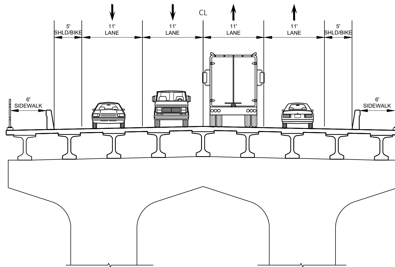
Oregon/Jackson Street Typical Section - Across Bridge
