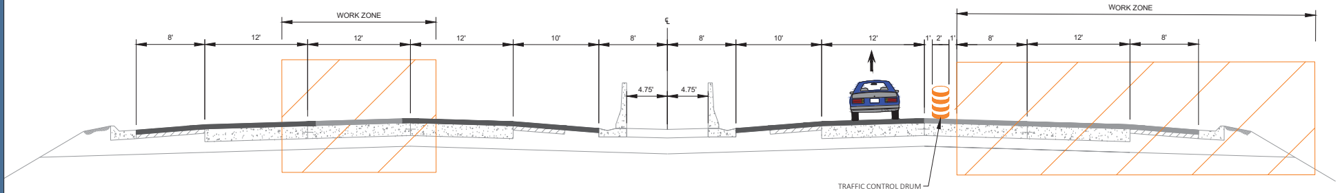
STAGE 3 (FULL NORTHBOUND CLOSURE - NIGHT TIME)
