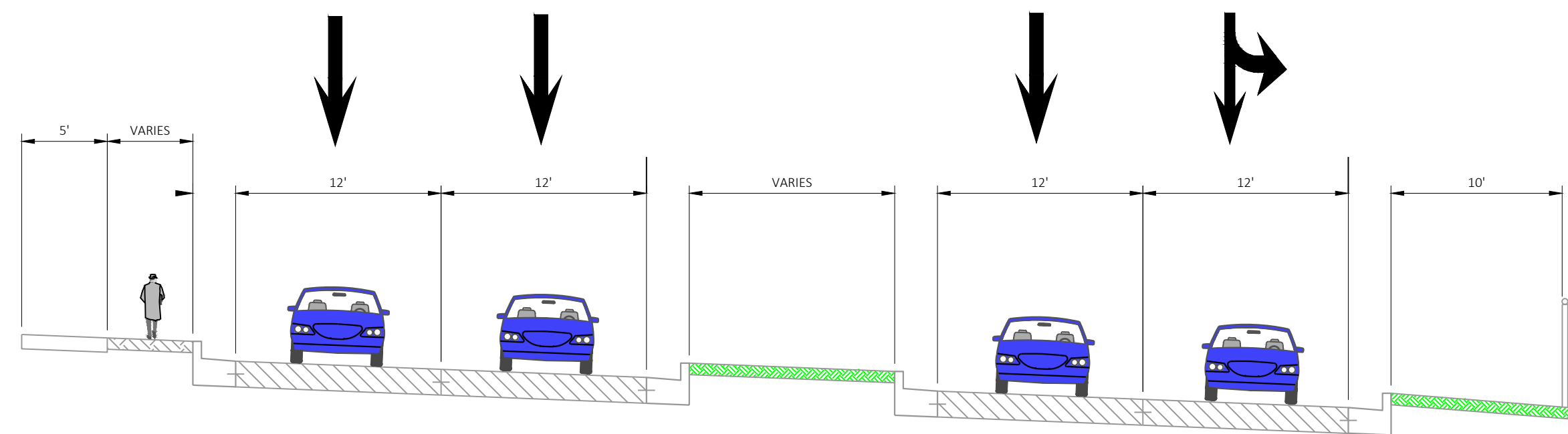
EXISTING TYPICAL SECTION SOUTHBOUND RAMPS & 5TH ST
