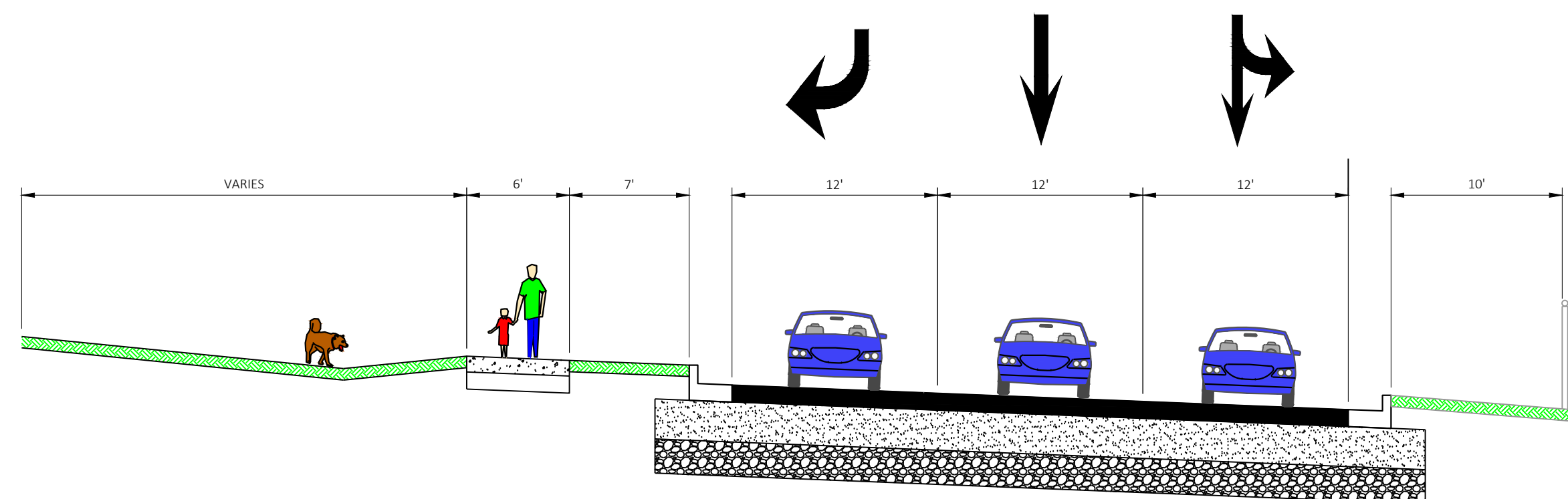
PROPOSED TYPICAL SECTION SOUTHBOUND RAMPS & 5TH ST
