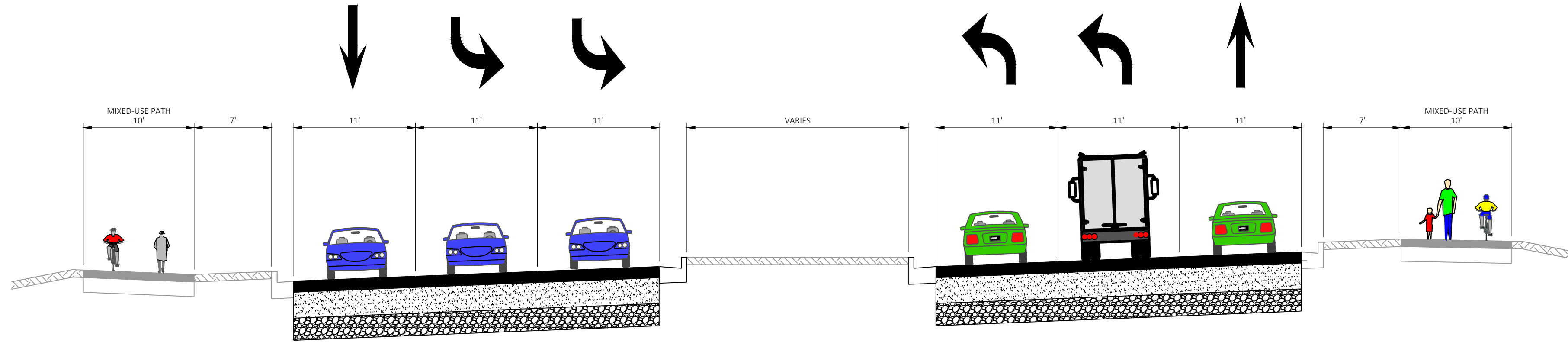
EXISTING TYPICAL SECTION BECHER ST
