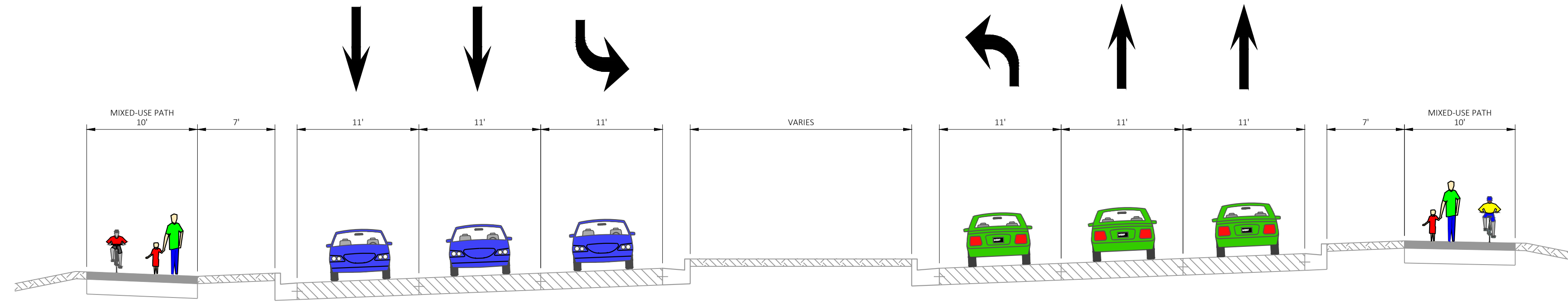
EXISTING TYPICAL SECTION BECHER ST
