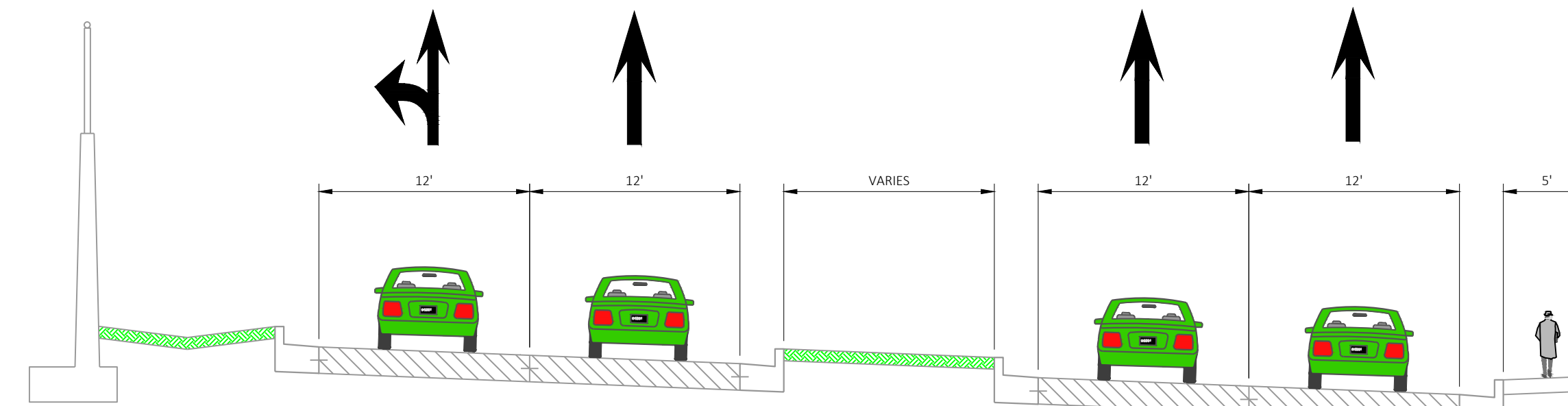
EXISTING TYPICAL SECTION NORTHBOUND RAMPS & 4TH ST
