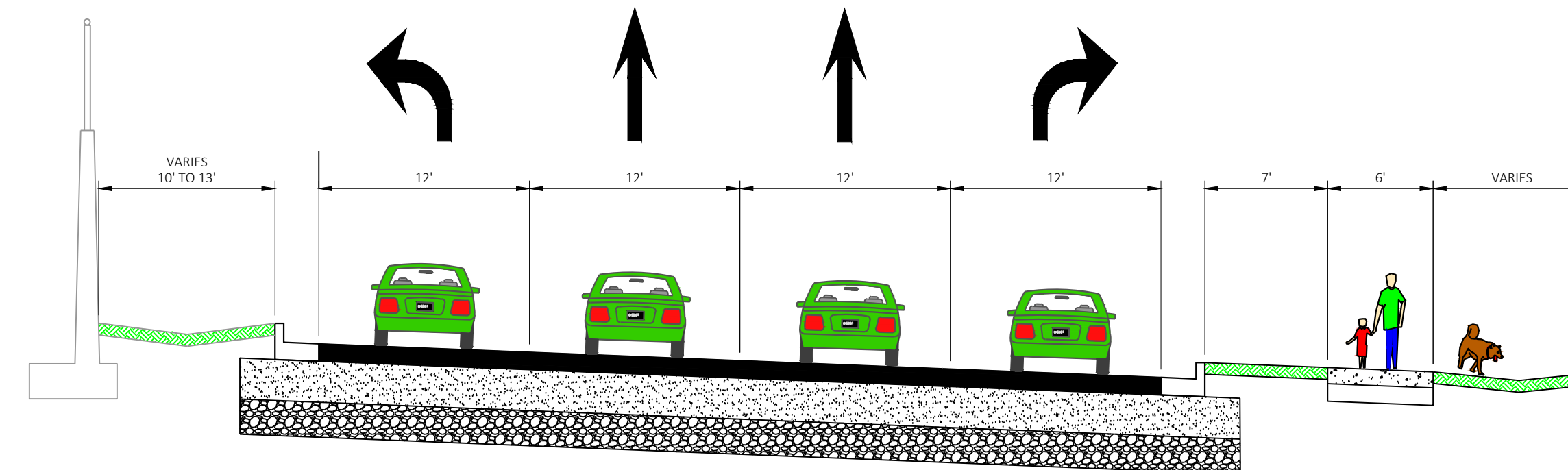
PROPOSED TYPICAL SECTION NORTHBOUND RAMPS & 4TH ST
