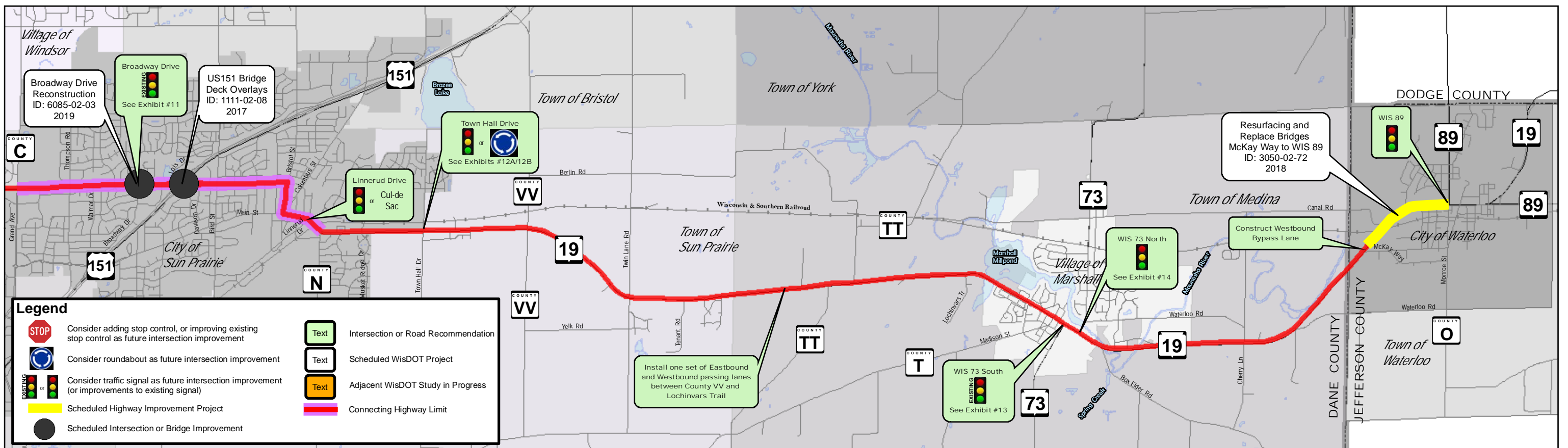
SRH Consulting Group, Inc. WIS 19 Safety and Operations Study - Improvement Overview - (Primary Recommendations) US 12 to WIS 89 (Dane and Jefferson Counties) Project ID: 5290-00-09
