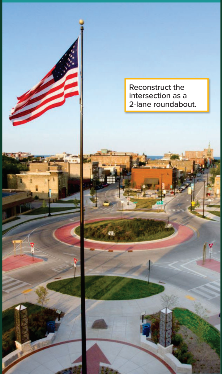
Urban Roundabout Example: WIS 20/32 (7th St), Racine, WI
