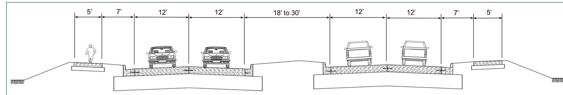
Proposed Typical Section: Yahara River Bridge to Larson Beach Road
