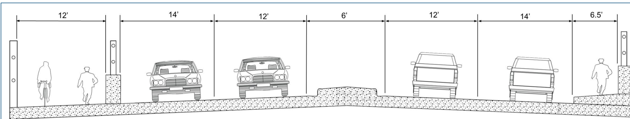
Proposed Typical Section: Yahara River Bridge
