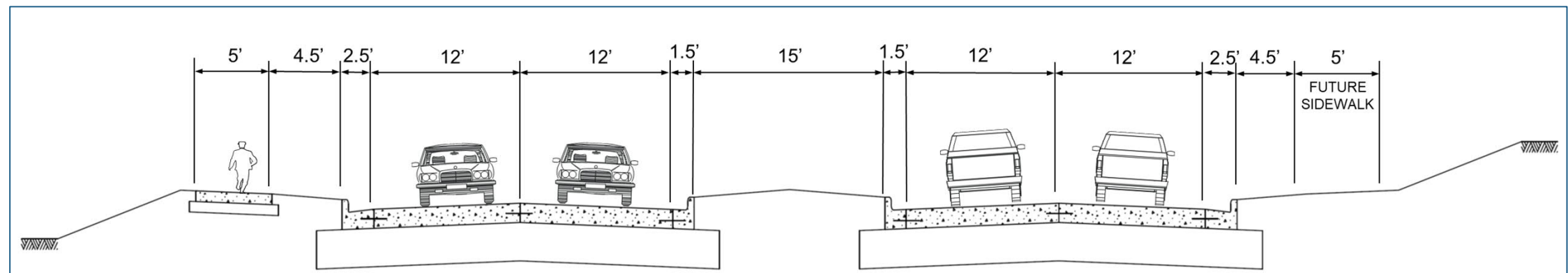
Proposed Typical Section: Exchange Street to Yahara River Bridge
