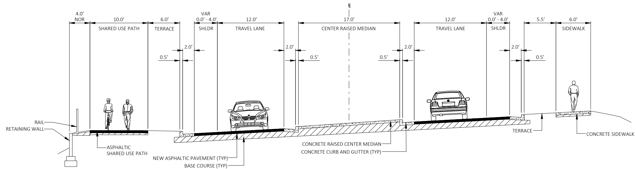
TYPICAL FINISHED SUPERELEVATED SECTION - ALTERNATIVE 1 SUNNYSIDE DRIVE TO US 14/US 61
