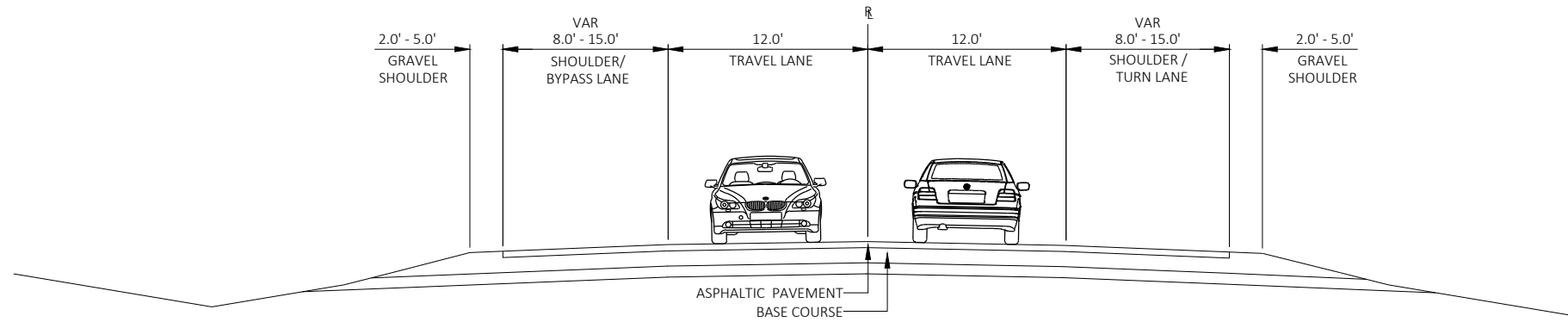
TYPICAL EXISTING SECTION LA CROSSE CO LINE TO RIVERVIEW DRIVE
