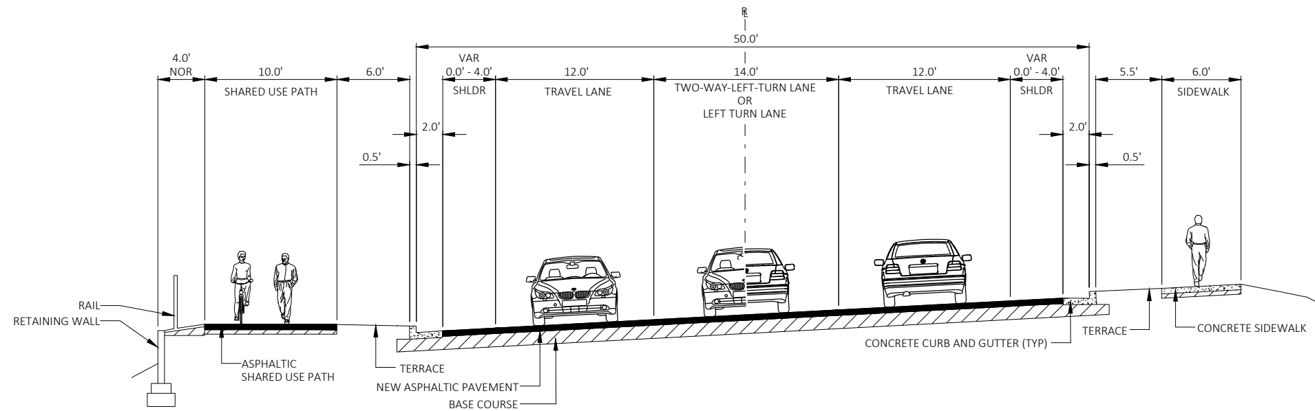
TYPICAL FINISHED SUPERELEVATED SECTION - ALTERNATIVE 2 SUNNYSIDE DRIVE TO US 14/US 61 (STH 35 SOUTH)
