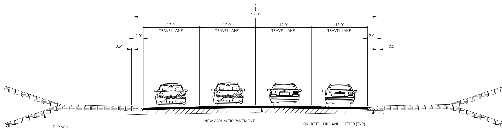
TYPICAL FINISHED SECTION US 14/US 61
