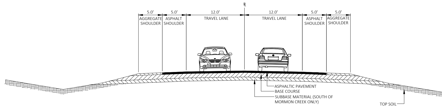
TYPICAL FINISHED SECTION LA CACROSSE CO LINE TO SUNNYSIDE DRIVE
