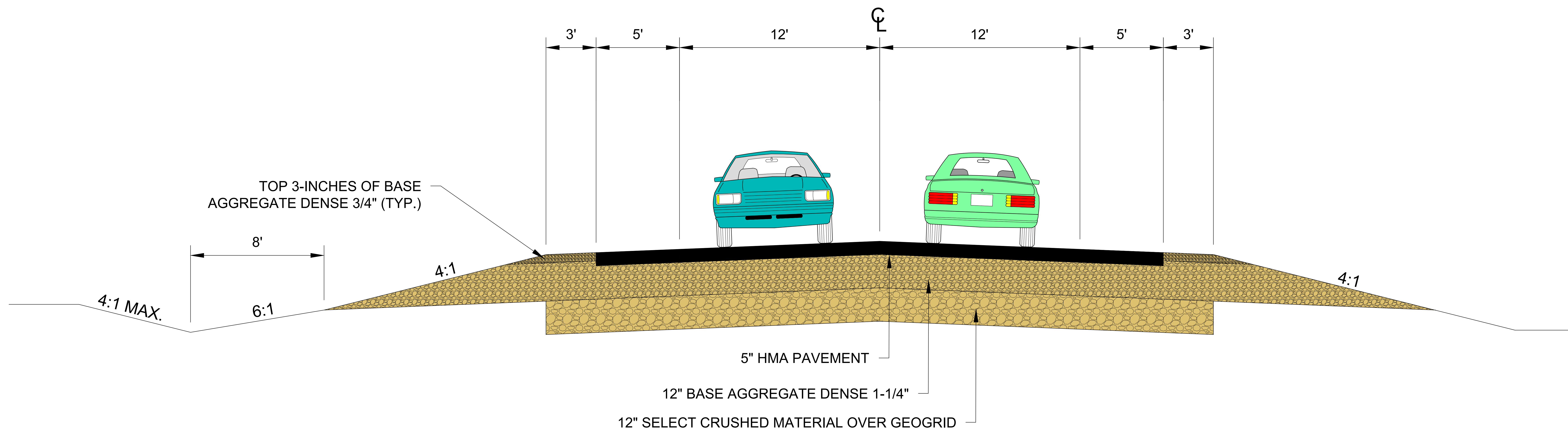
PROPOSED RURAL SECTION
