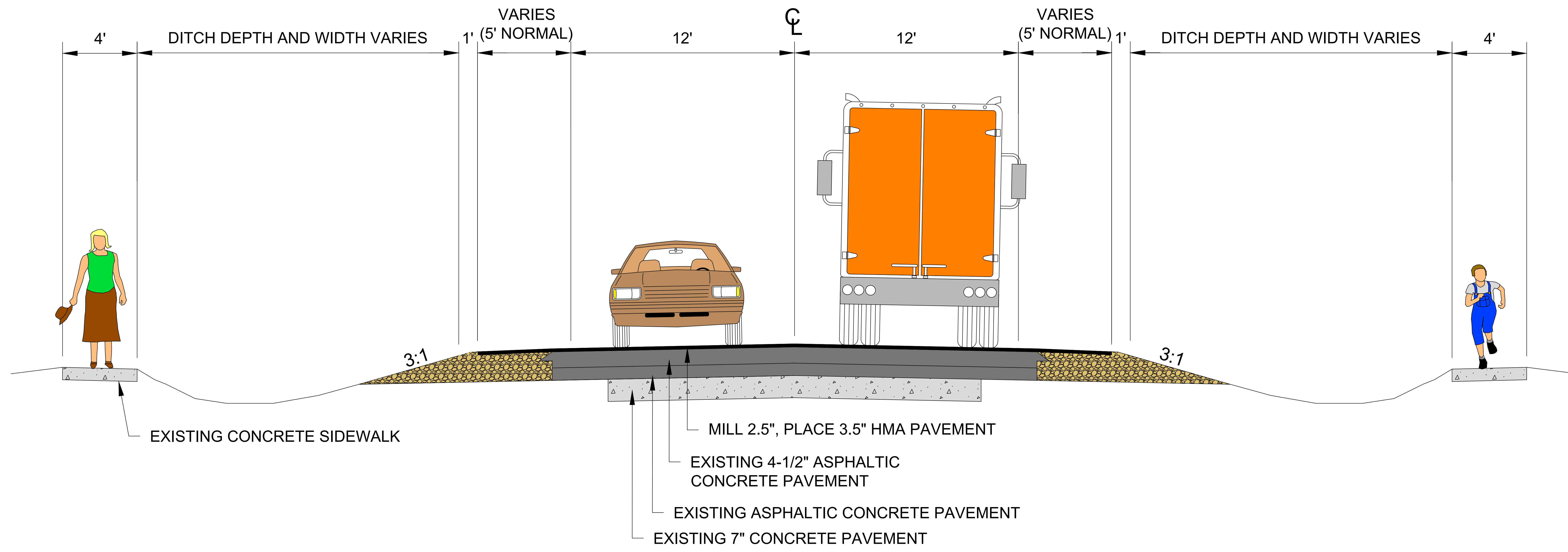
PROPOSED URBAN SECTION
