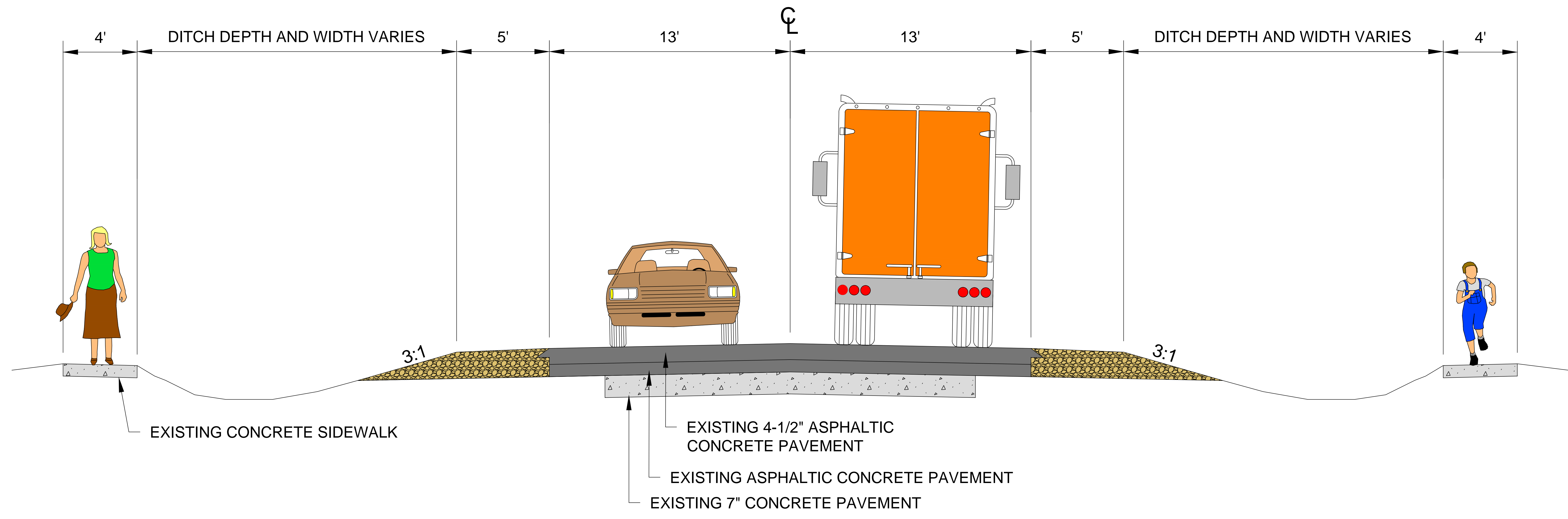
EXISTING URBAN SECTION
