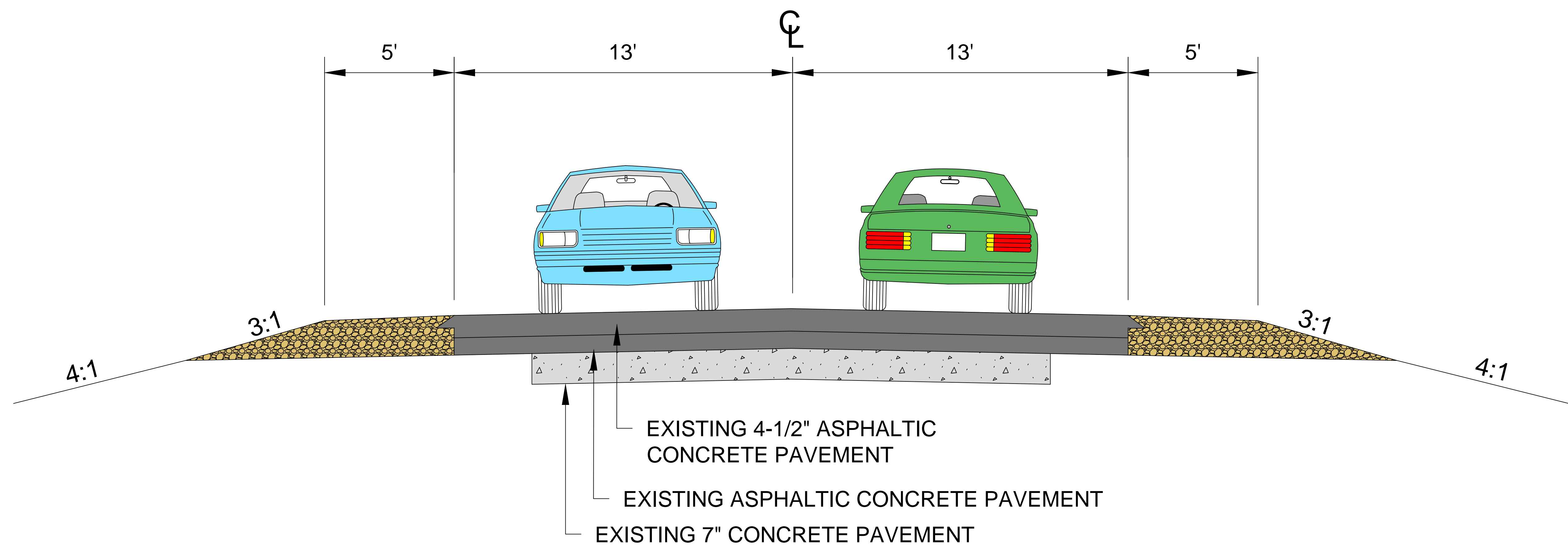
EXISTING RURAL SECTION
