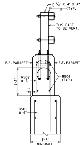
SECTION C-C
