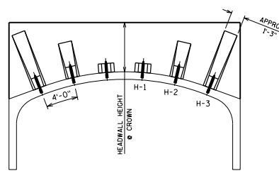
SAMPLE ELEVATION
