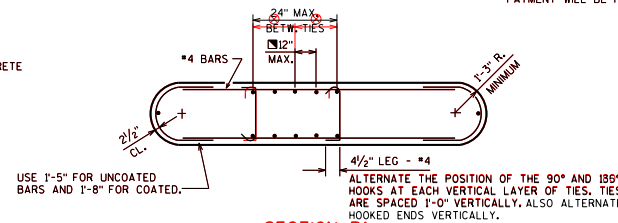
SECTION B1
