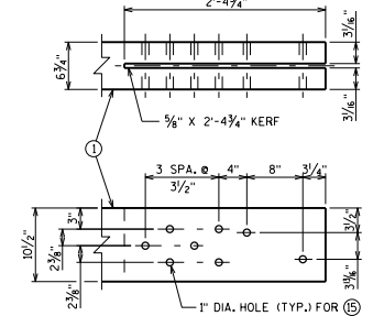
TRANSITION GLULAM RAIL BORING DETAIL
