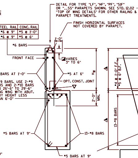
SECTION A2 ALL WING LENGTHS
