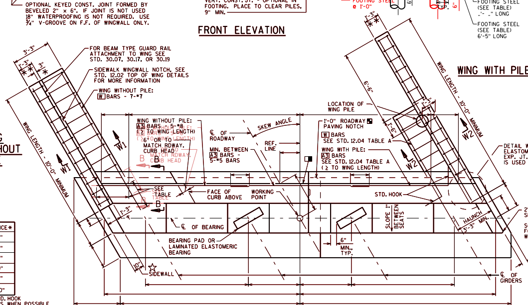
WING WITH SIDEWALK
