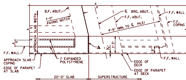
APPROACH SLAB PARTIAL PLAN * (AT WINGWALLS PARALLEL TO BRIDGE - BRG ABUT - A1 ABUT. - SLAB SPAN)
