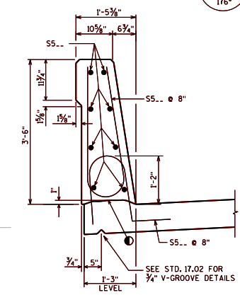
SECTION THRU PARAPET ON BRIDGE
