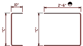
⑥ DUCT STIRRUP #4 AT 9" MAX. (16) EACH GIRDER END (12) EACH GIRDER DUCT
