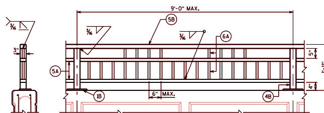
TYPE C4
