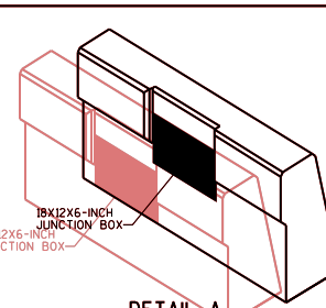
DETAIL A SHOWING B.F. OF PARAPET WITH ANCHORAGE DETAILS SHOWING BLOCK OUT FOR JUNCTION BOX.
