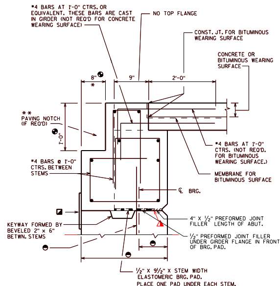
PRECAST DOUBLE TEE OR MULTI-STEM SECTION
