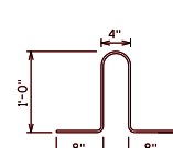
⑩ SHEAR CONNECTOR TIE ONE LEG OF BAR TO ③ EPOXY COAT BARS #4 AT 2'-0" MAX. (FOR SECTION 1)
