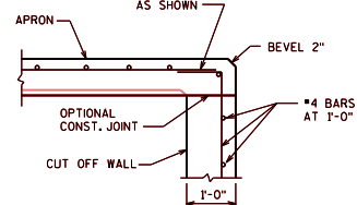
SECTION C6
