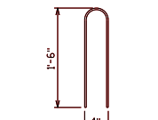
⑨ SHEAR CONNECTOR TIE ONE LEG OF BAR TO ③ EPOXY COAT BARS #4 AT 2'-0" MAX. (FOR SECTIONS 2-6)
