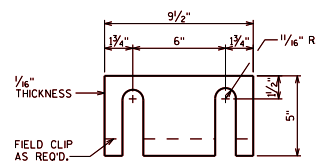
POST SHIM DETAIL 4 PER POST
