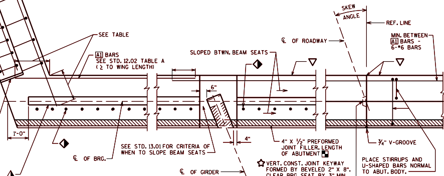
SLAB SPAN WITH FIXED SEAT
