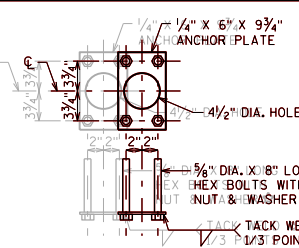
ANCHORAGE DETAIL
