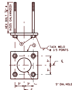
ANCHORAGE DETAIL
