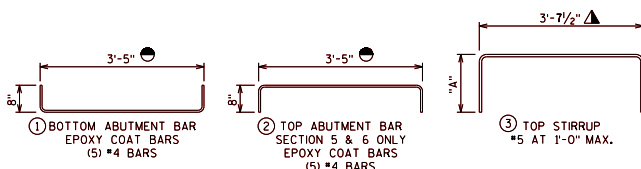
4'-0" SECTIONS
