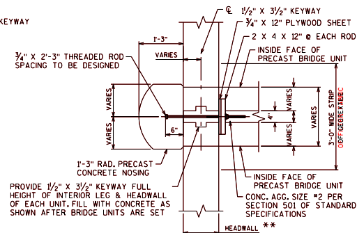
DETAIL 6B
