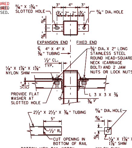
TOP RAIL CONNECTION FOR FENCE W/ BENT TOP
