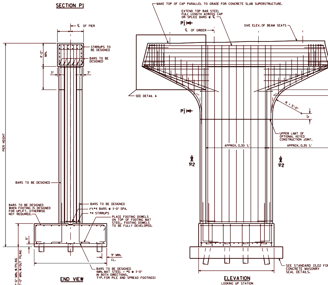
SECTION P1
