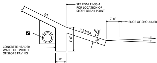
ALT. SECTION @ SHOULDER (RURAL ROADWAY)
