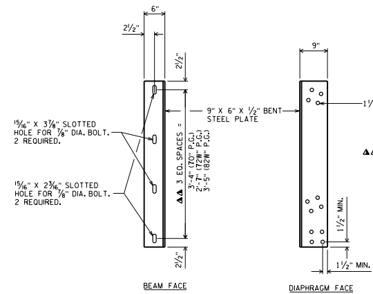
DIAPHRAGM SUPPORT
