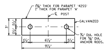
POST CLAMP SPACER DETAIL
