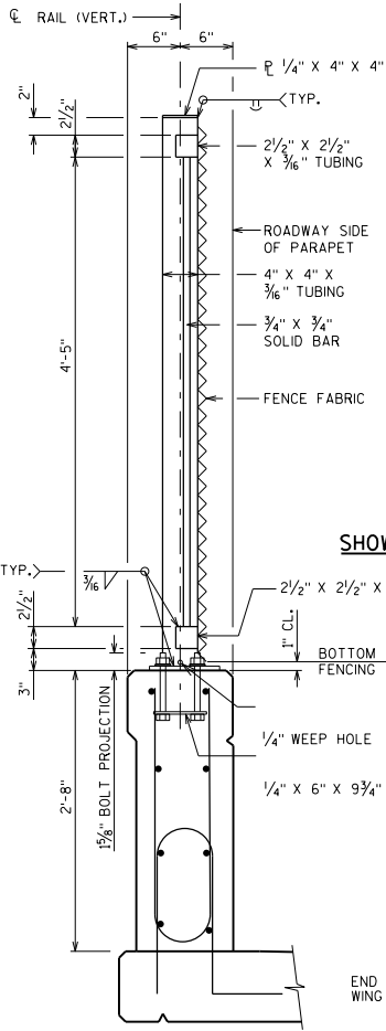
SECTION THRU RAILING (SEE STD. 30.07 FOR PARAPET REINFORCEMENT AND DETAILS)
