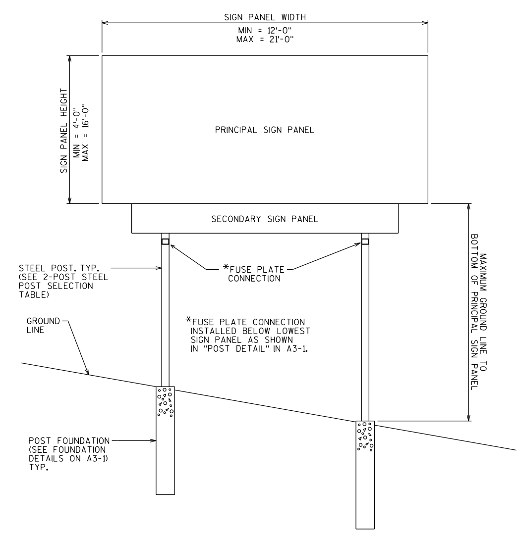
2-POST SIGN CONFIGURATION
