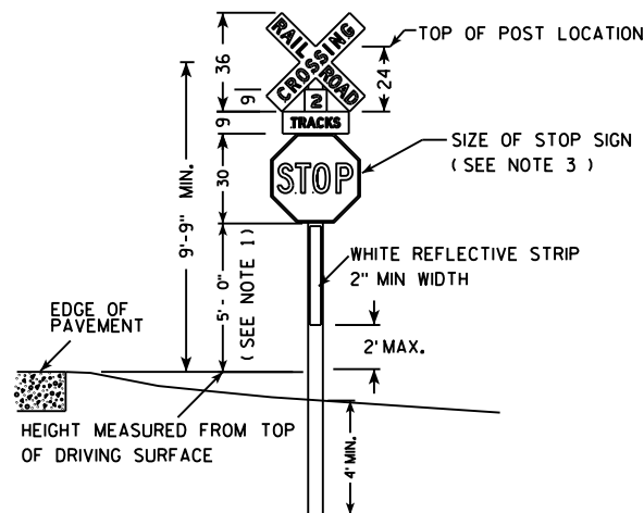
30" X 30" STOP SIGN
