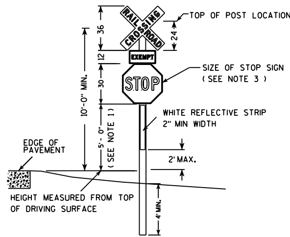
30" X 30" STOP SIGN
