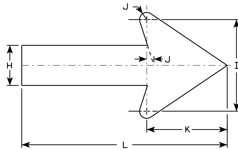
ARROW DETAIL
