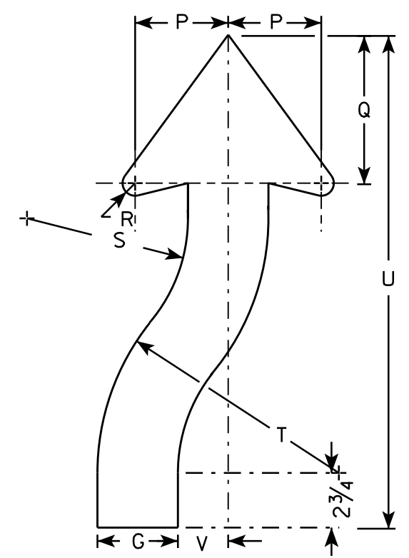
ARROW DETAIL
