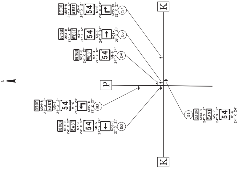
DETAIL 4 STAGE 2
