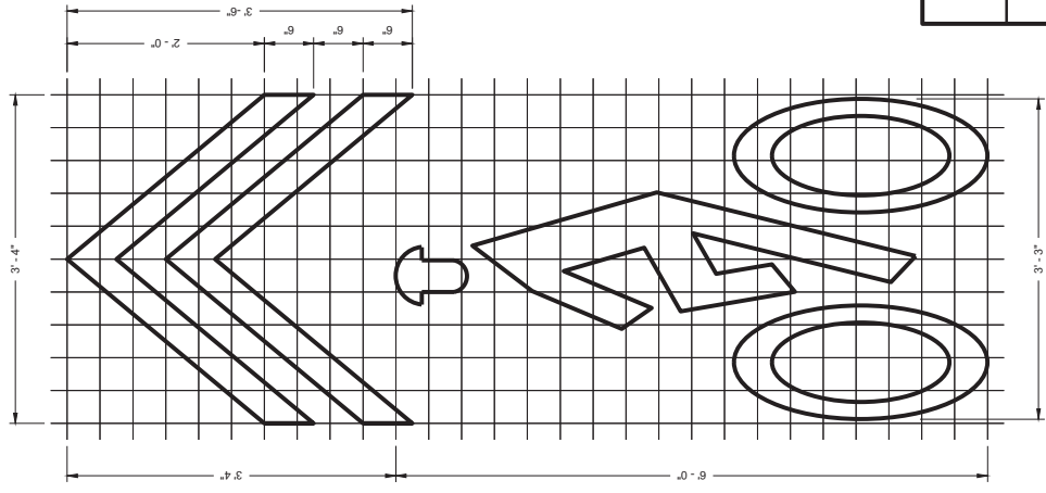
BIKE LANE SYMBOL FOR SHARED LANE
