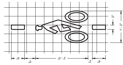
BICYCLE DETECTOR PAVEMENT MARKING
