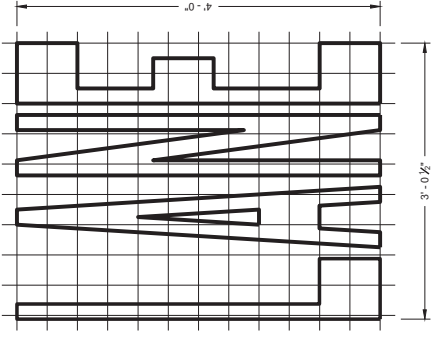
BIKE LANE WORDS
