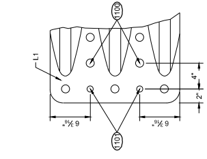
ELEVATION VIEW
