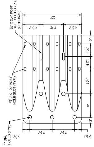
ELEVATION VIEW
