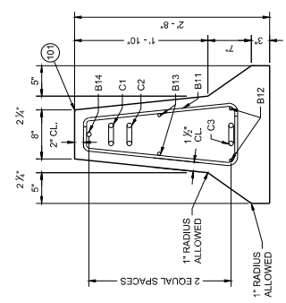
END SECTION
