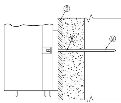
SIDE VIEW ASPHALT ANCHOR INSTALLATION THROUGH ASPHALT OVERLAY ON TOP OF CONCRETE PAVEMENT
