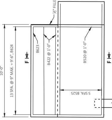
WING 3 ELEVATION (BACK FACE)
