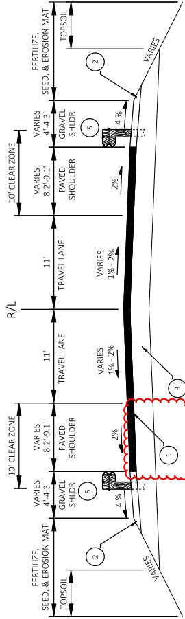
PROPOSED TYPICAL SECTION WEST ZINDA DRIVE (CTH C) STA 8+60.00 TO STA 8+62.05 STA 10+67.97 TO STA 11+18.00
