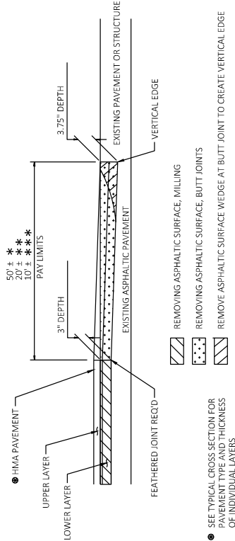
BUTT JOINT DETAIL FOR MILLED ASPHALTIC PAVEMENTS (PROFILE CHANGE)
