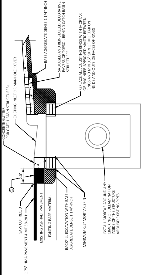
RECONSTRUCTING CATCH BASINS AND MANHOLES
