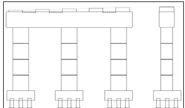
WisDOT BOS Standard Detail (2015)
