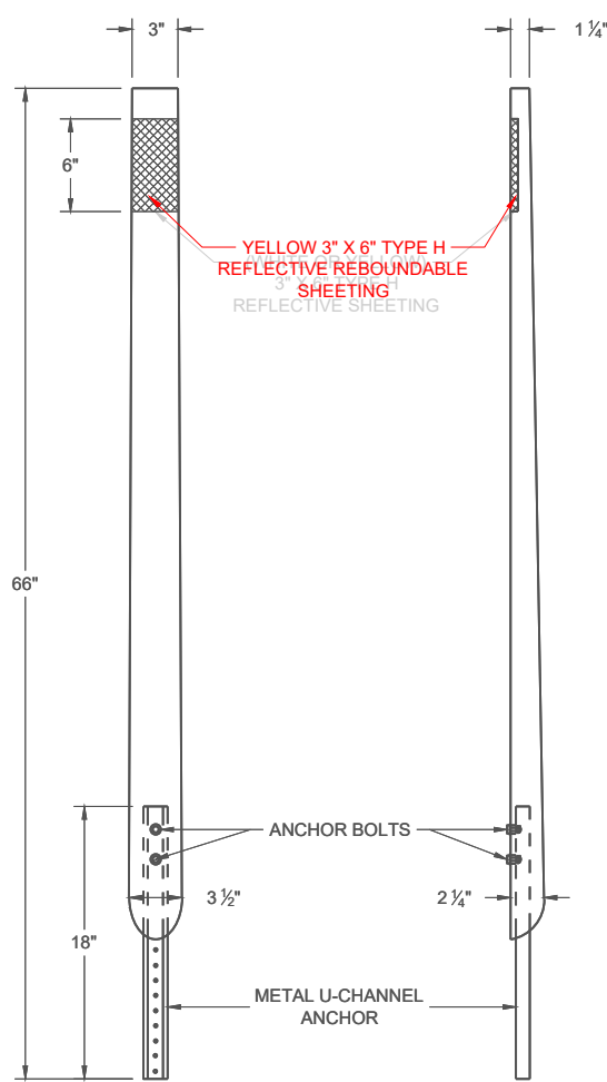
FRONT VIEW SIDE VIEW ALTERNATE 2 FLEXIBLE DELINEATOR POSTS
