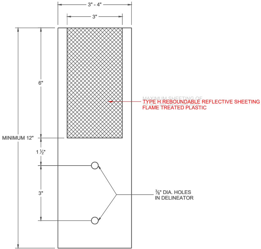
4' x 12' DELINEATOR WITH REFLECTIVE SHEETING GUARDRAIL REFLECTOR
