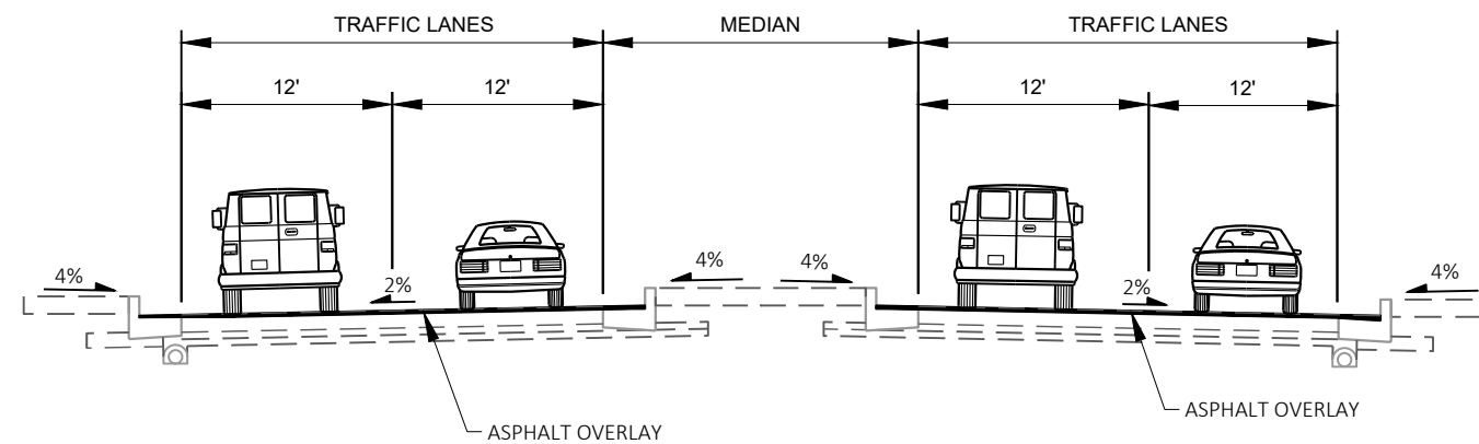
FINISHED 4-LANE DIVIDED TYPICAL SECTION - WIS 107
