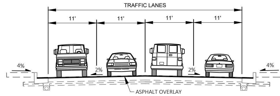
FINISHED 4-LANE UNDIVIDED TYPICAL SECTION - WIS 107
