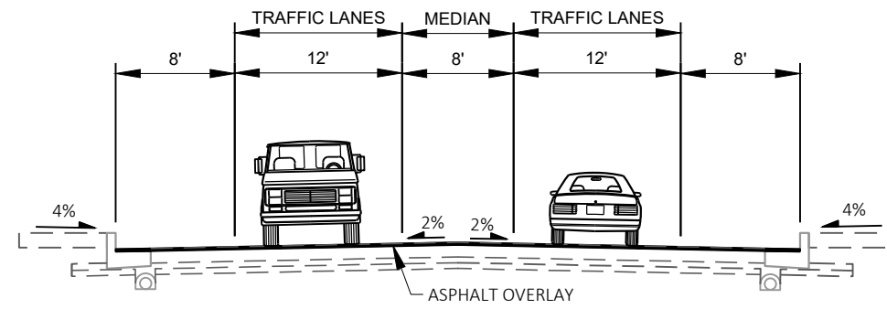
FINISHED 4-LANE UNDIVIDED TYPICAL SECTION - WIS 107
