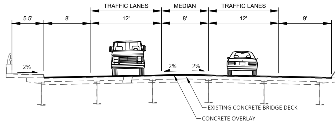
FINISHED 4-LANE UNDIVIDED BRIDGE TYPICAL SECTION - WIS 107 B-37-239, B-37-240
