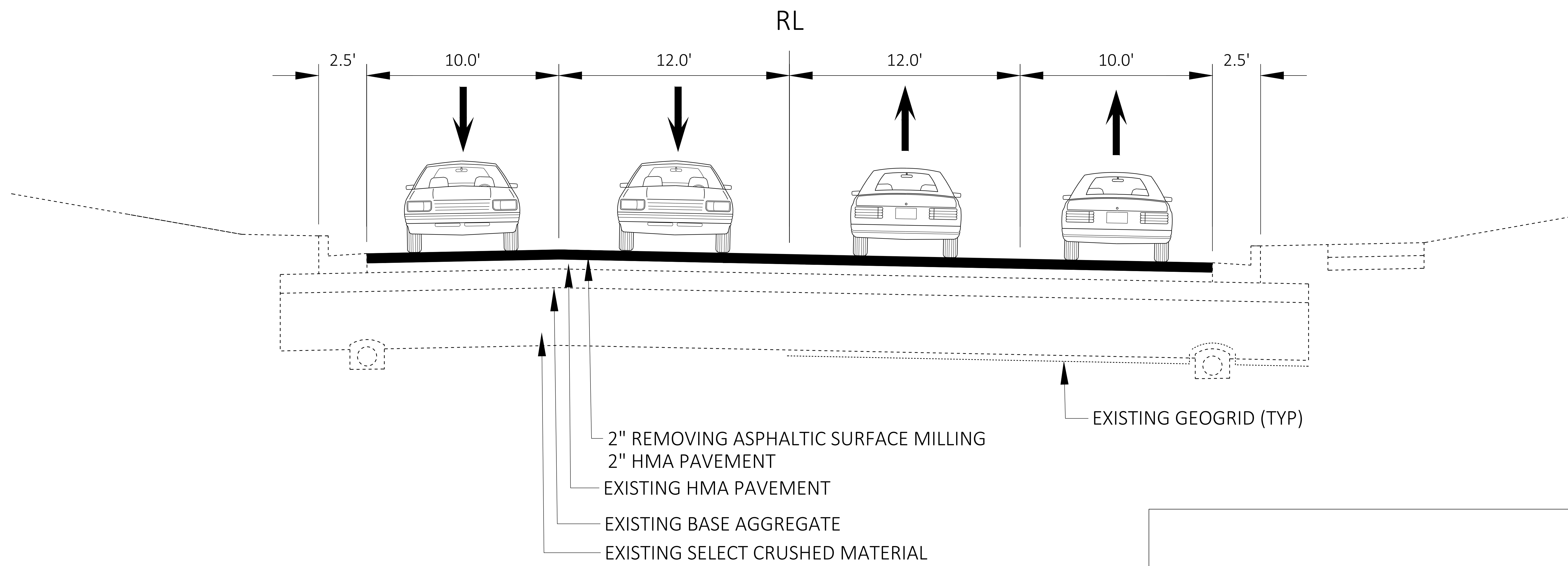
TYPICAL FINISHED SECTION MONROE ST TO NORTH ST
