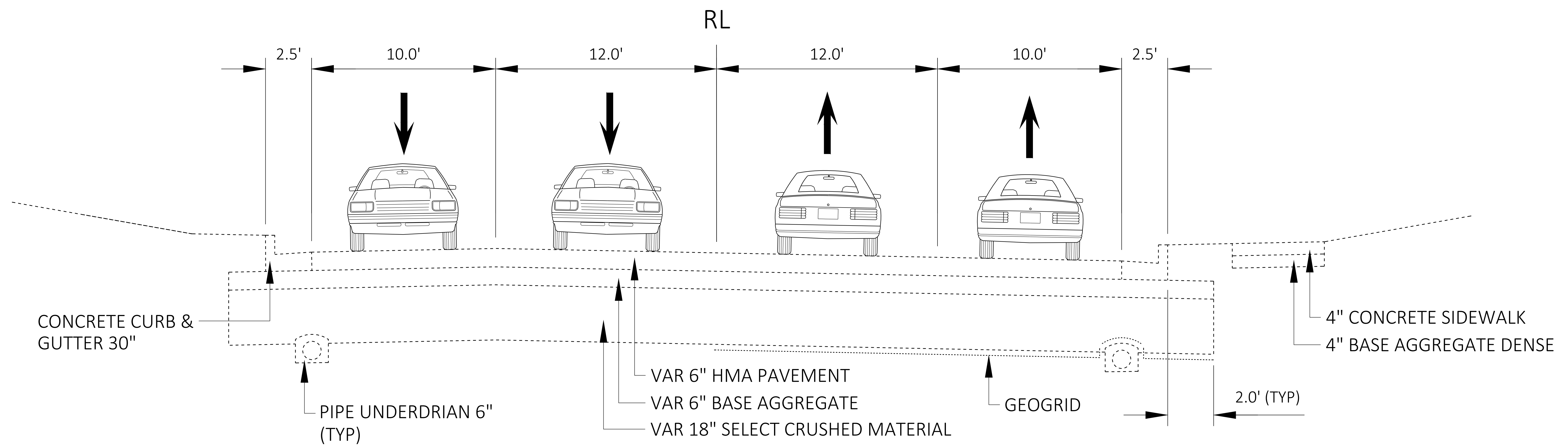
TYPICAL EXISTING SECTION MONROE ST TO NORTH ST
