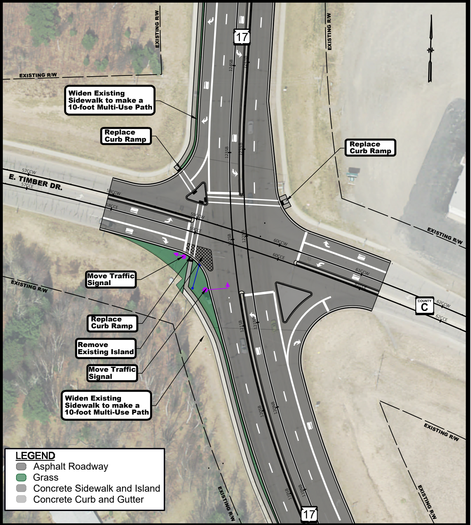
Plan View
