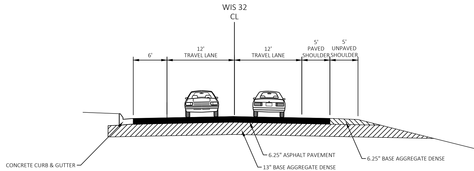
EXISTING TYPICAL SECTION WIS 32 FOURTH STREET TO SIXTH STREET LOOKING NORTH
