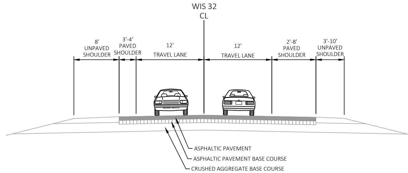
EXISTING TYPICAL SECTION WIS 32 FOURTH STREET TO SIXTH STREET LOOKING NORTH
