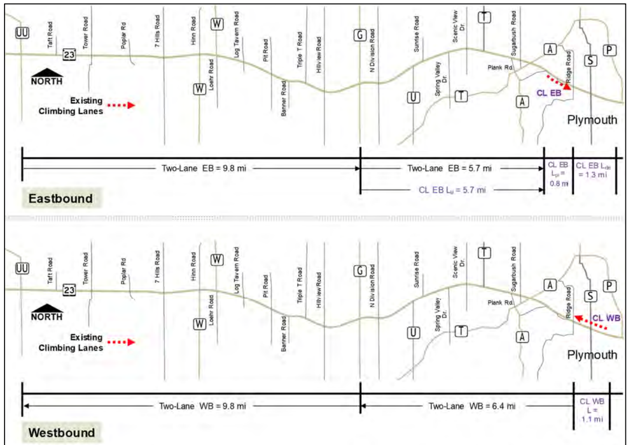
Figure 4: 2017 and 2040 No-Build Alternative : Two-Lane Highway Analysis Sections
