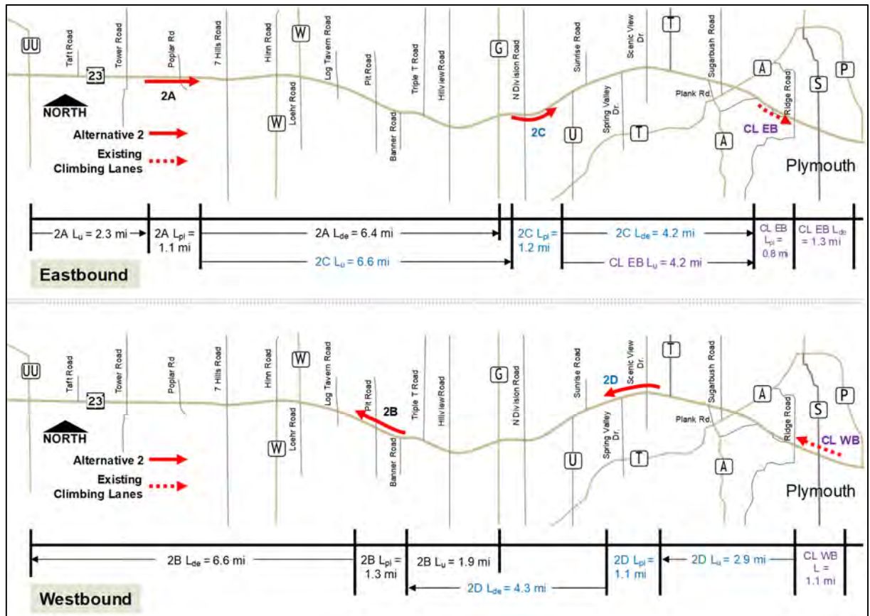
Figure 5: Passing Lane Alternative: Two-Lane Highway Analysis Sections
