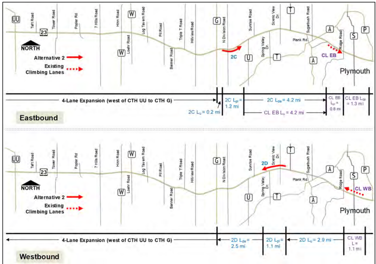
Figure 6: Hybrid Alternative: Two-Lane Analysis Sections
