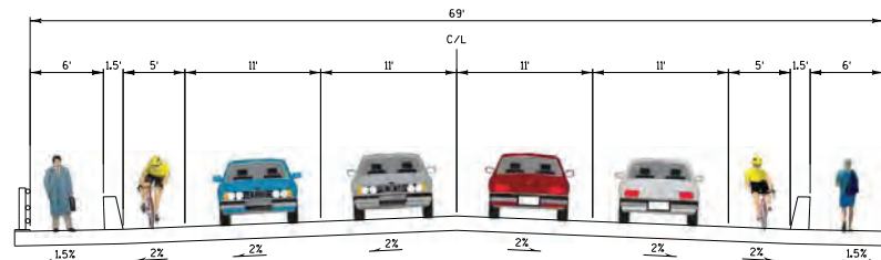
RECONSTRUCTED TYPICAL SECTION WITH BARRIER
