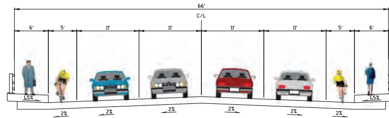
RECONSTRUCTED TYPICAL SECTION WITHOUT BARRIER
