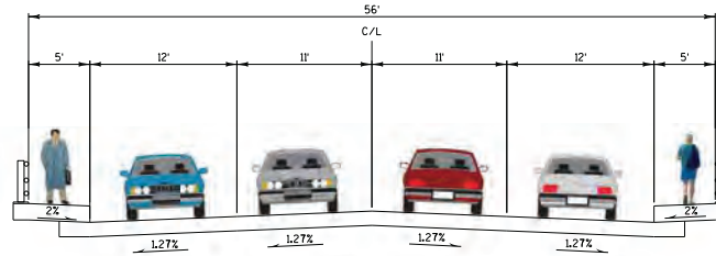
REHABILITATED EXISTING TYPICAL SECTION
