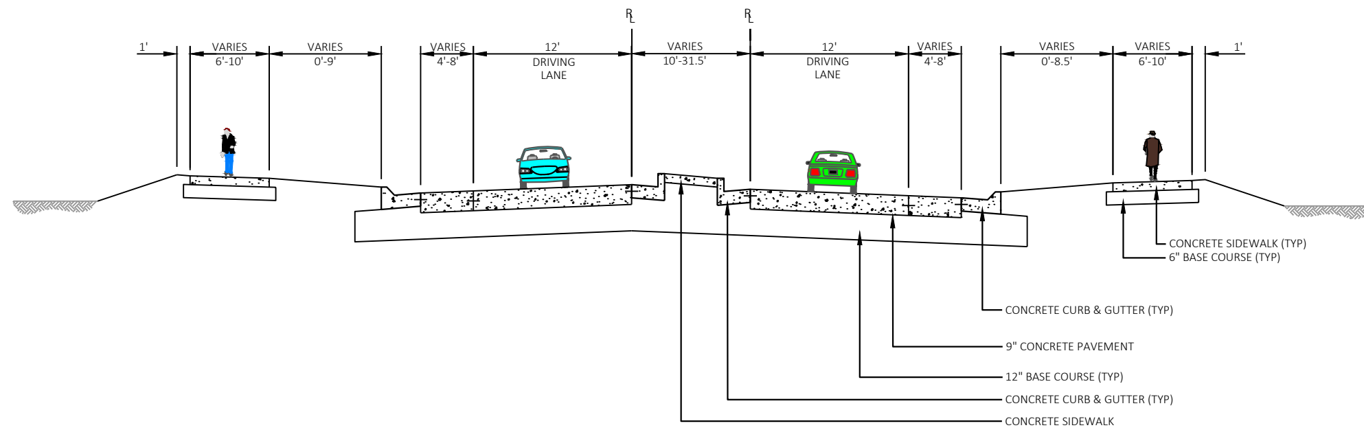
TYPICAL FINISHED SECTION US 10 & WIS 25
