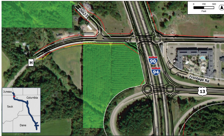
Split Diamond Interchange Alternative
