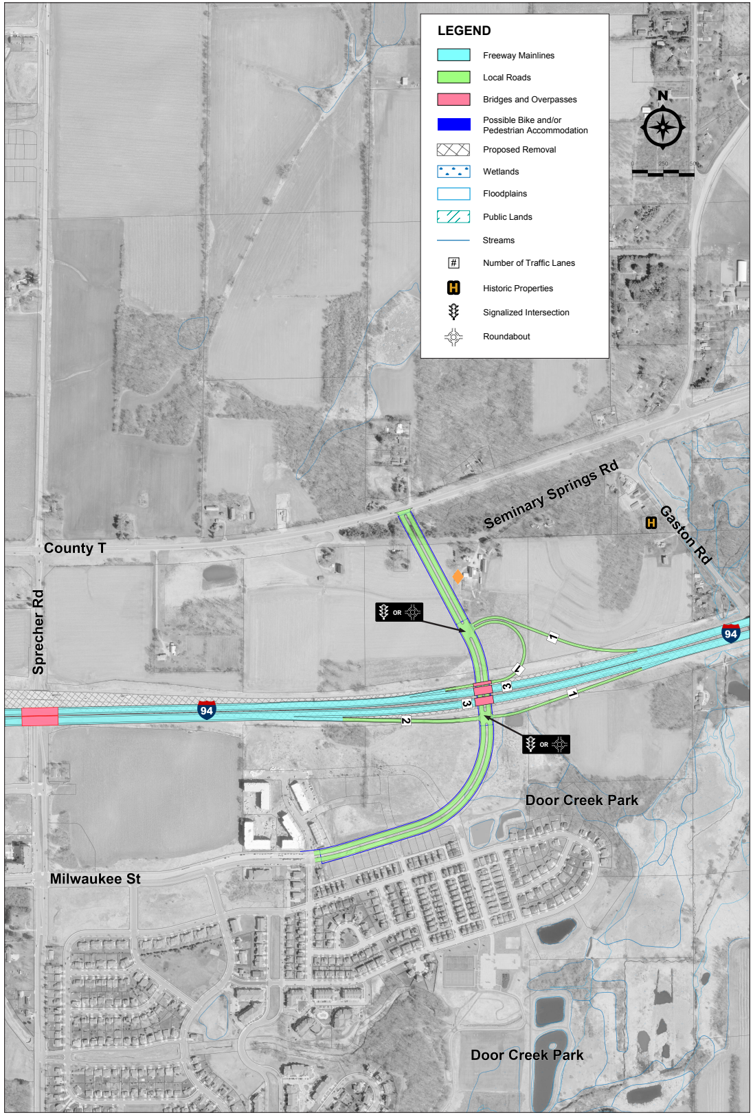
Bike and pedestrian accommodations, including sidewalk, are intended to be installed as shown here, pending community agreement, final design considerations, and ability to acquire real estate.
