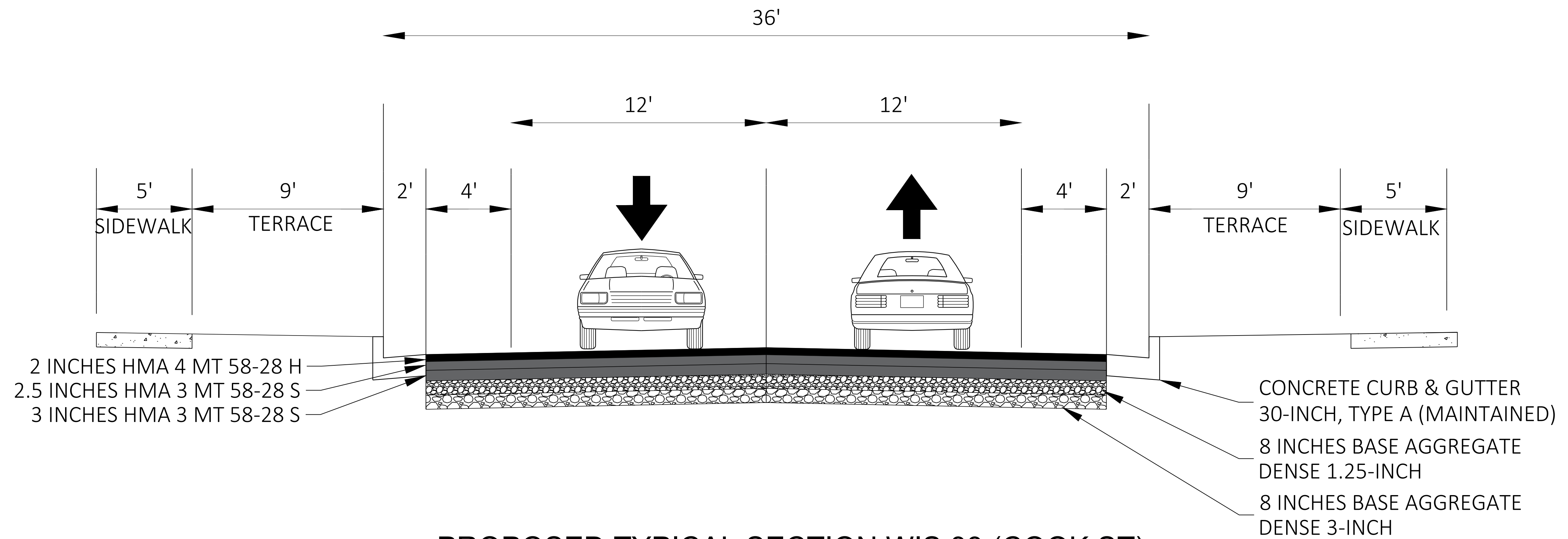
PROPOSED TYPICAL SECTION WIS 33 (COOK ST)
