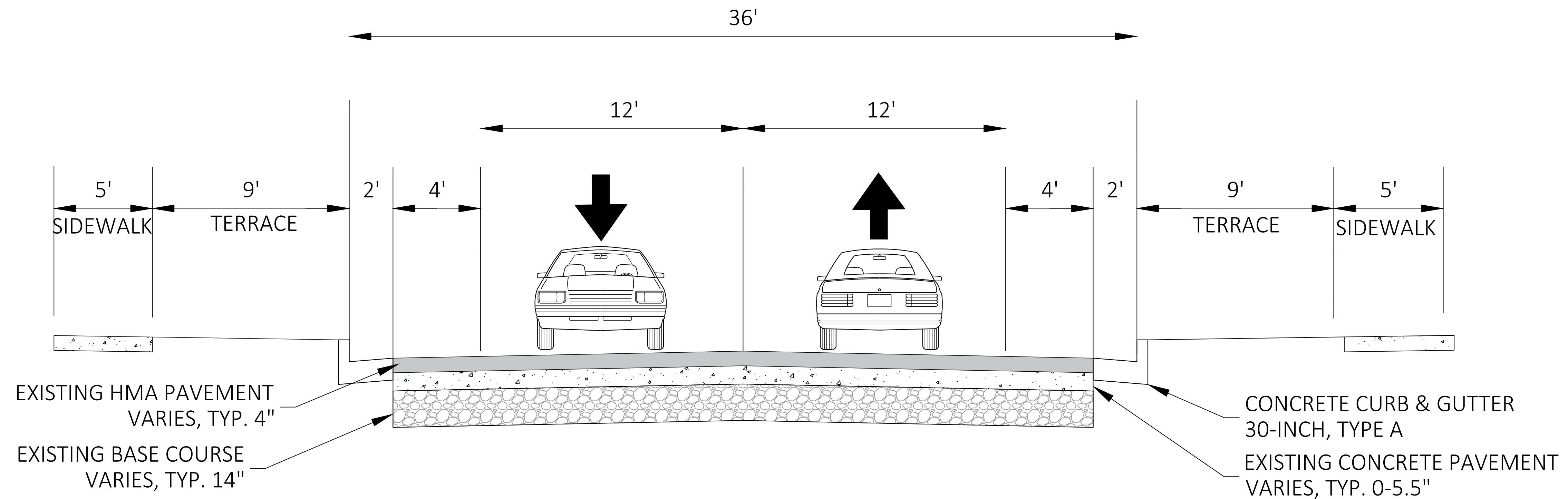
EXISTING TYPICAL SECTION WIS 33 (COOK ST)
