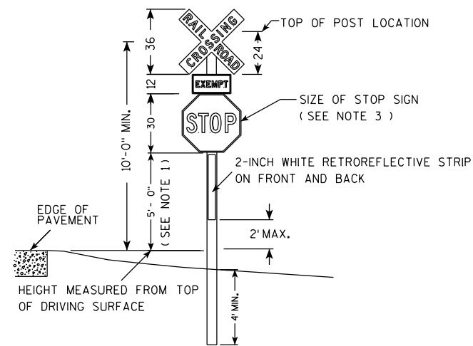
30" X 30" STOP SIGN
