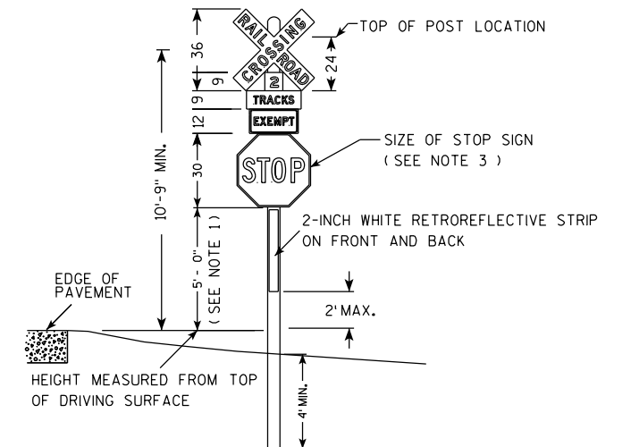
30" X 30" STOP SIGN
