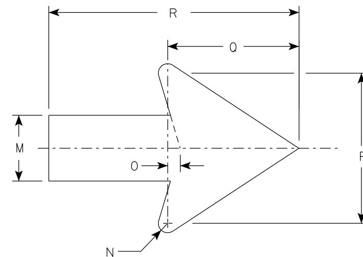
Arrow Detail
