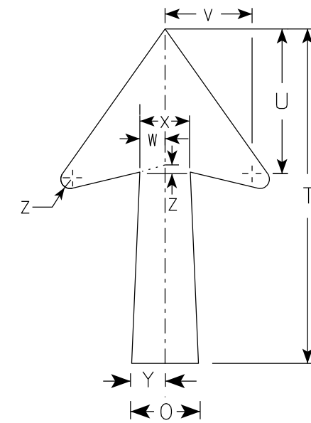
Arrow Detail
