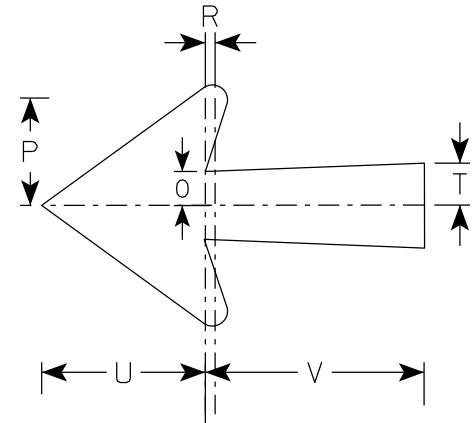
Arrow Detail
