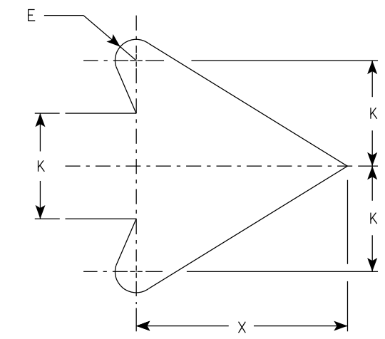
ARROW DETAIL
